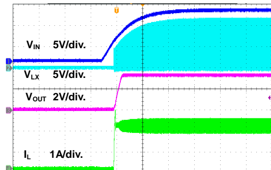
Figure 13. Startup Through Power Supply Waveform
